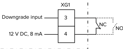
Fig. 13: Schematic circuit diagram: Connection of an external switching contact (default setting: NC)
